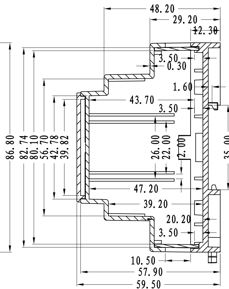
SEC B-B
