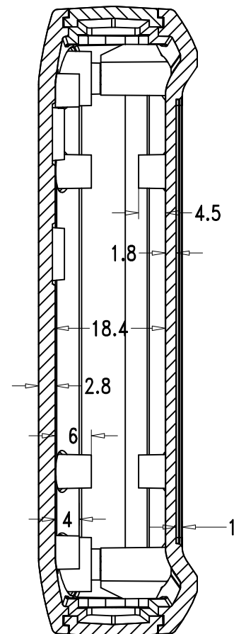
SEC B-B
