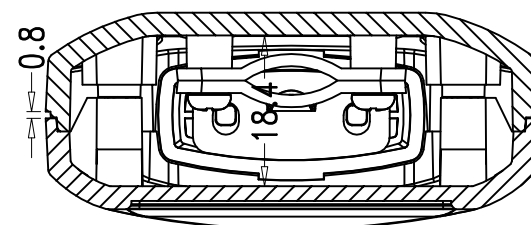
SEC B-B
