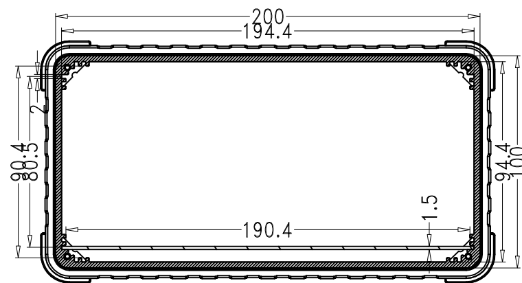
SEC B-B
