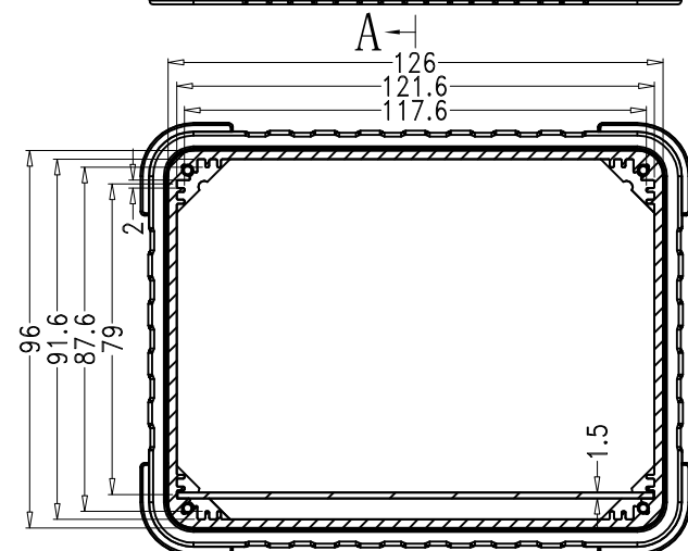
SEC B-B
