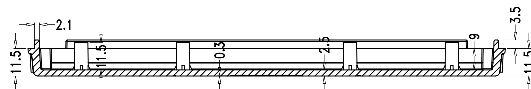
SEC B-B
