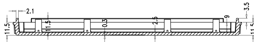
SEC B-B
