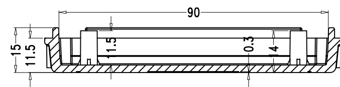
SEC B-B
