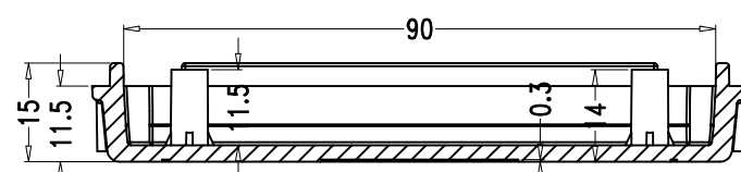
SEC B-B
