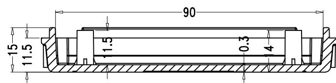
SEC B-B
