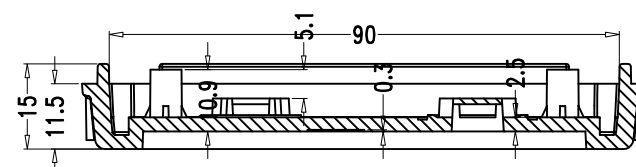
SEC B-B
