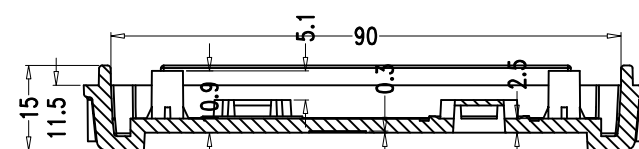
SEC B-B
