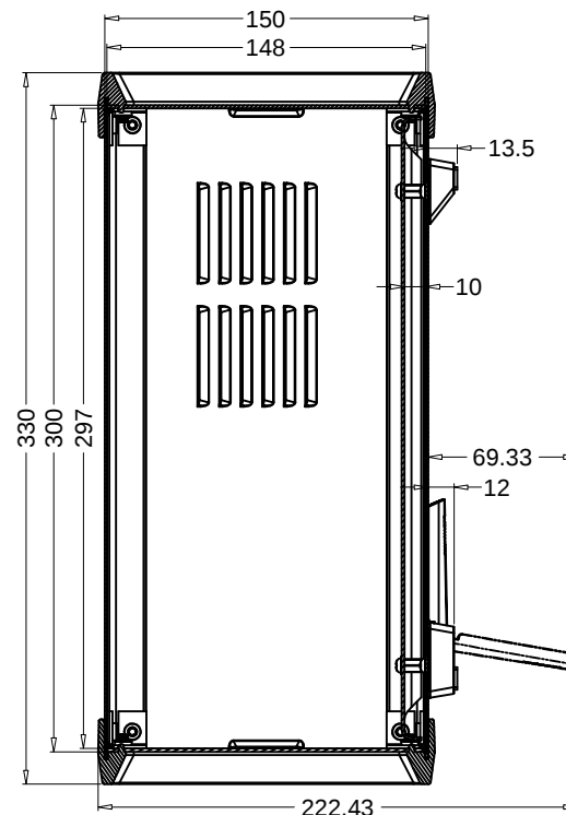
SEC B-B
