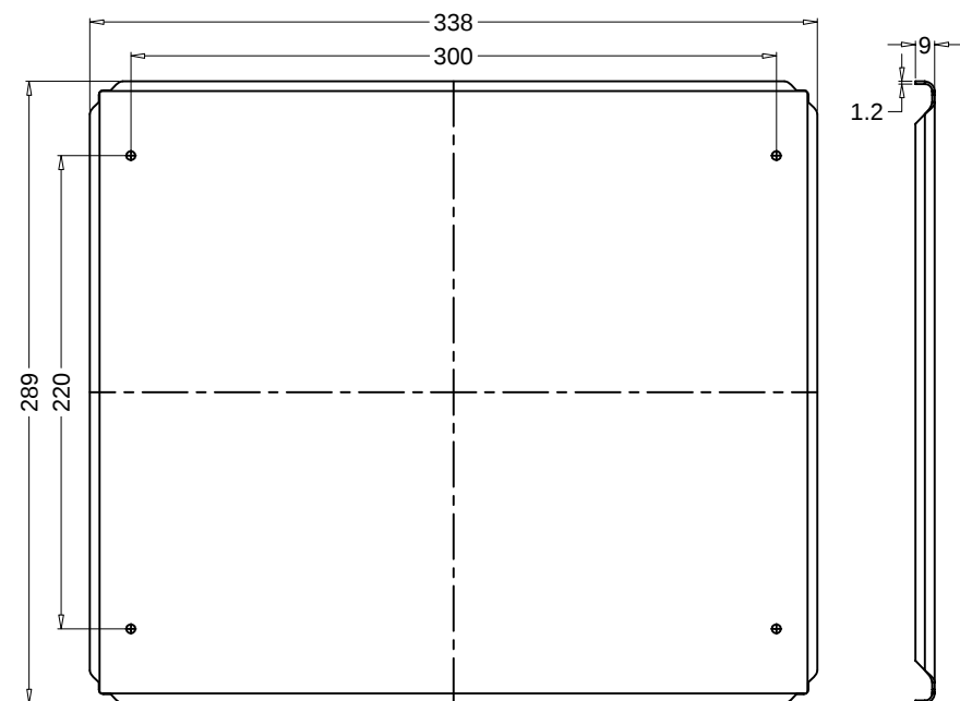
Lining plate
