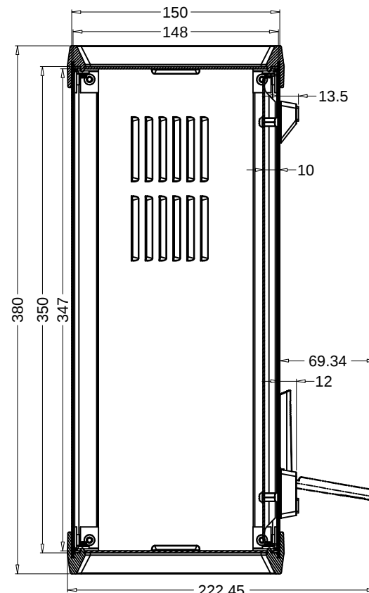
SEC B-B
