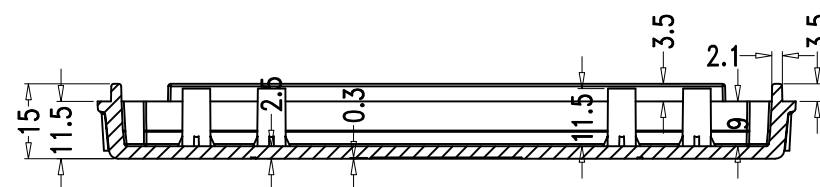
SEC B-B
