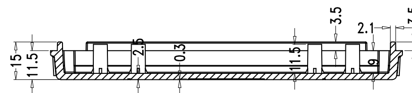
SEC B-B
