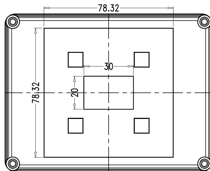
SEC B-B
