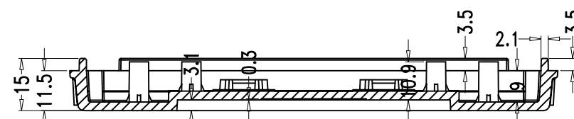
SEC B-B
