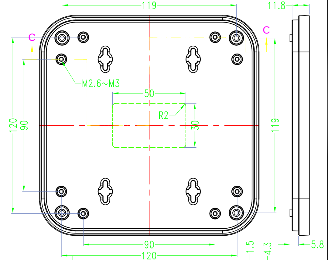
SEC C-C
